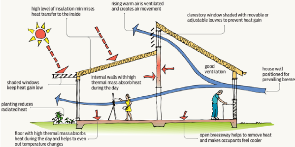
Figure 5-9: Overall Passive Design Strategies
