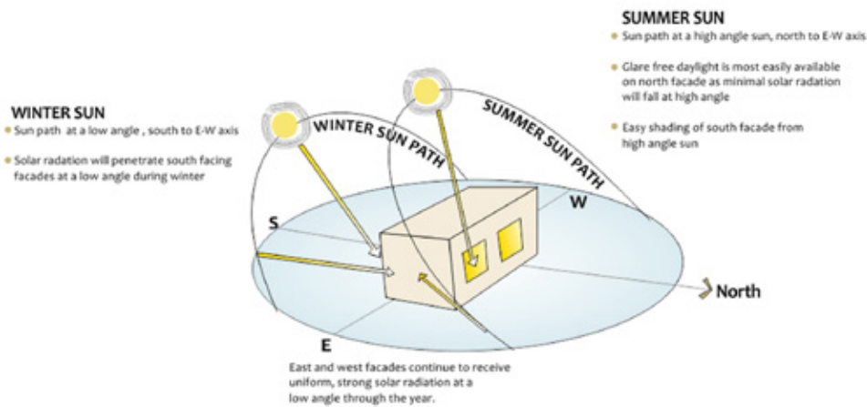
Figure 5-4: Orientation of Longer Axis of Building along North and South
