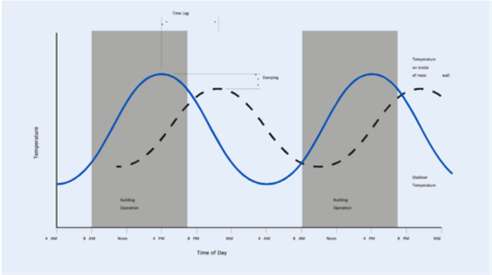
Figure 7-2: Temperature Swing
