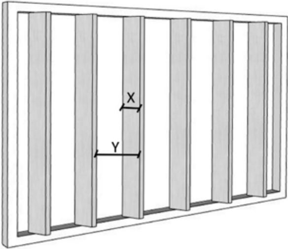
Figure 4-4: Vertical Shading or Louvres (Relationship Between Depth (x) and Gap (y): x \geq 0.234y )
