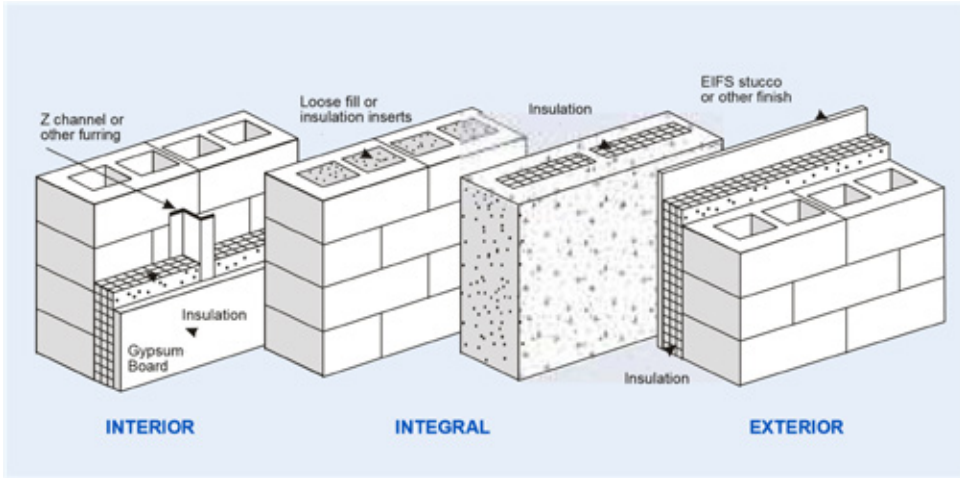
Figure 7-3: Construction of Mass Walls of Buildings
