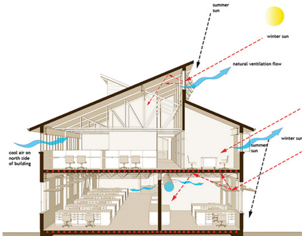
Figure 5-1: Building Section Showing Cross Ventilation
