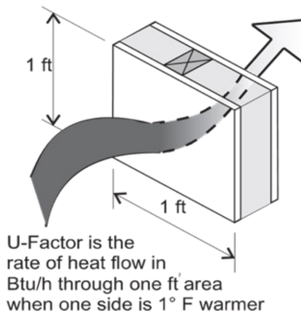
Figure 7-1: Conceptual Representation of U-factor
