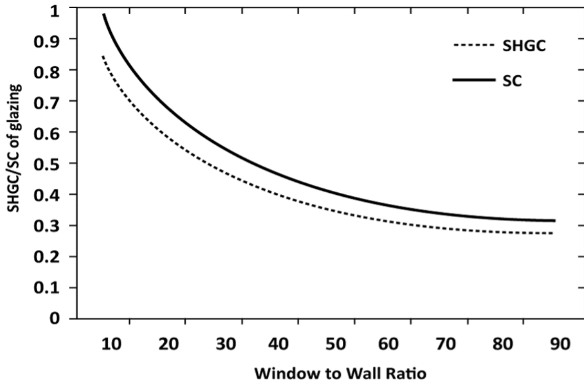
Figure 4-1: Selection of Glazing SHGC Based on WWR
