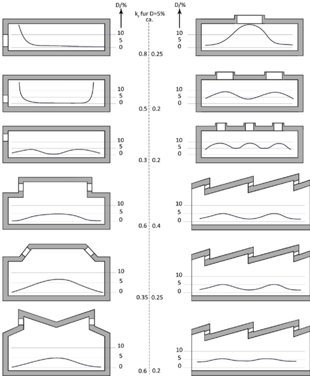
Figure 4-5: Influence of Windows and Skylights on Daylight Factor 1
