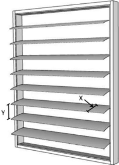
Figure 4-3: Horizontal Louvres (Relationship between depth (x) and gap (y): x \geq 0.234y )
