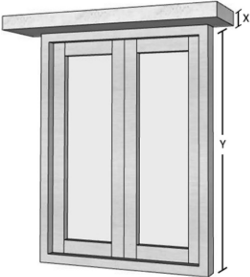
Figure 4-2: Horizontal Shade ( x \geq 0.234y )
