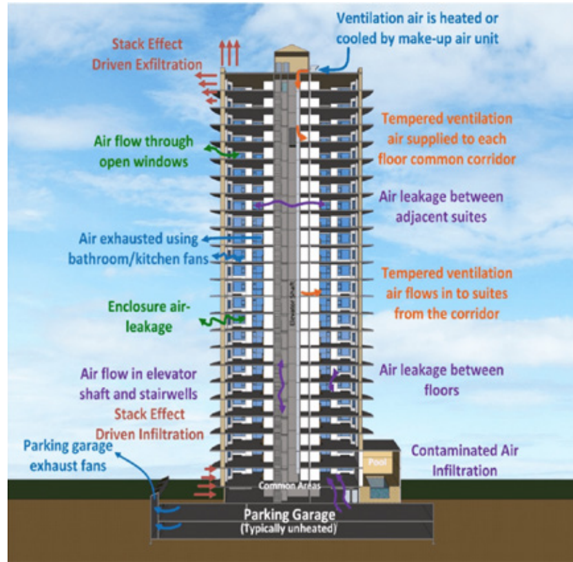
Figure 5-2: High-rise Building Section Showing Stack Ventilation
