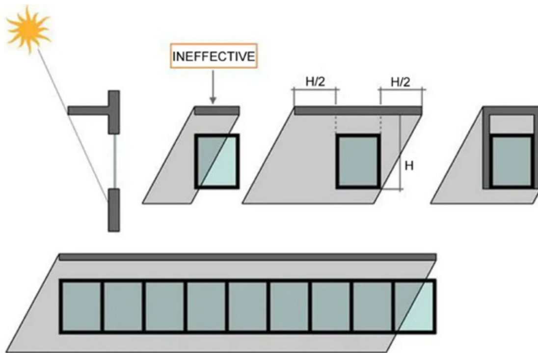
Figure 5-5: Façade Design with External Shading
